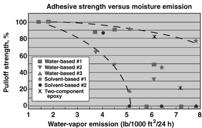
Fig. 8.3—Pulloff test results for different adhesives on concrete slabs with different moisture vapor emission rates (Suprenant and Malisch 1999a). (Note: 1 lb/1000 ft²/24 h = 0.488 kg/100 m²/24 h.)
