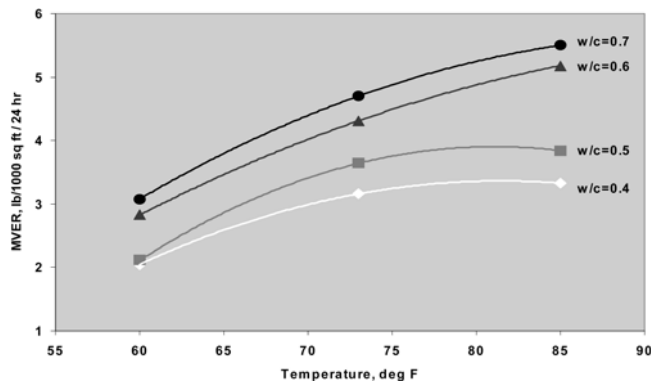
Fig. 3.10—Effect of temperature on calcium chloride emission tests for different concretes (Kanare 2005). (Note: 1\text{ }^{\circ}\text{F} = [(^{\circ}\text{F} - 32)/1.8]\text{ }^{\circ}\text{C} ; 1\text{ lb}/1000\text{ ft}^2/24\text{ h} = 0.488\text{ kg}/100\text{ m}^2/24\text{ h} .)
